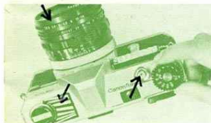
3. Shutter speed and aperture setting.
