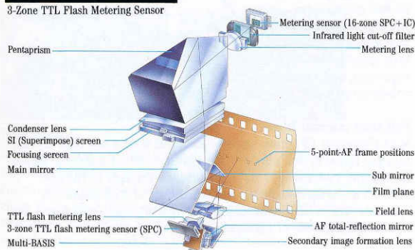
3-Zone TTL Flash Metering Sensor
