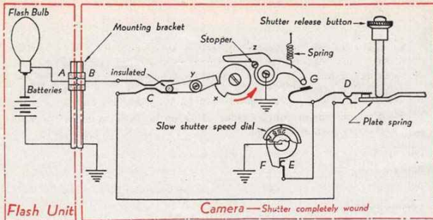
Schematic Diagram of Canon Model IV and IV-F BUILT-IN FLASH SYNCHRONIZER *
