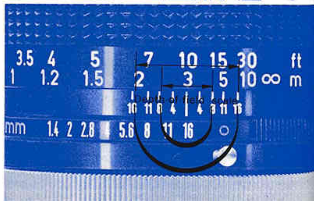
50mm Lens f/16 Depth-of-field 1.9m-7.6m (6'-25') Focused at 3m (10')
