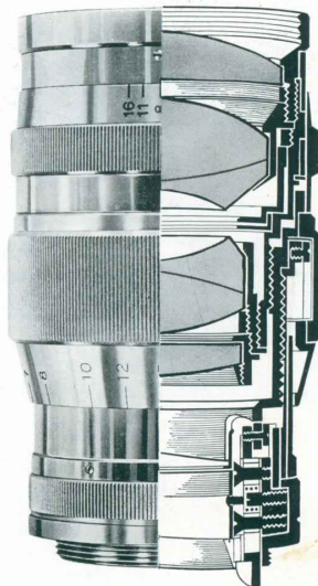
Cut-away-view of SERENAR 85mm f:2
